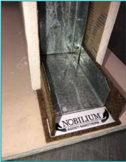
"Dry" thermo-acoustic application with 3 mm Nobilium® Thermalpanel for structures.
